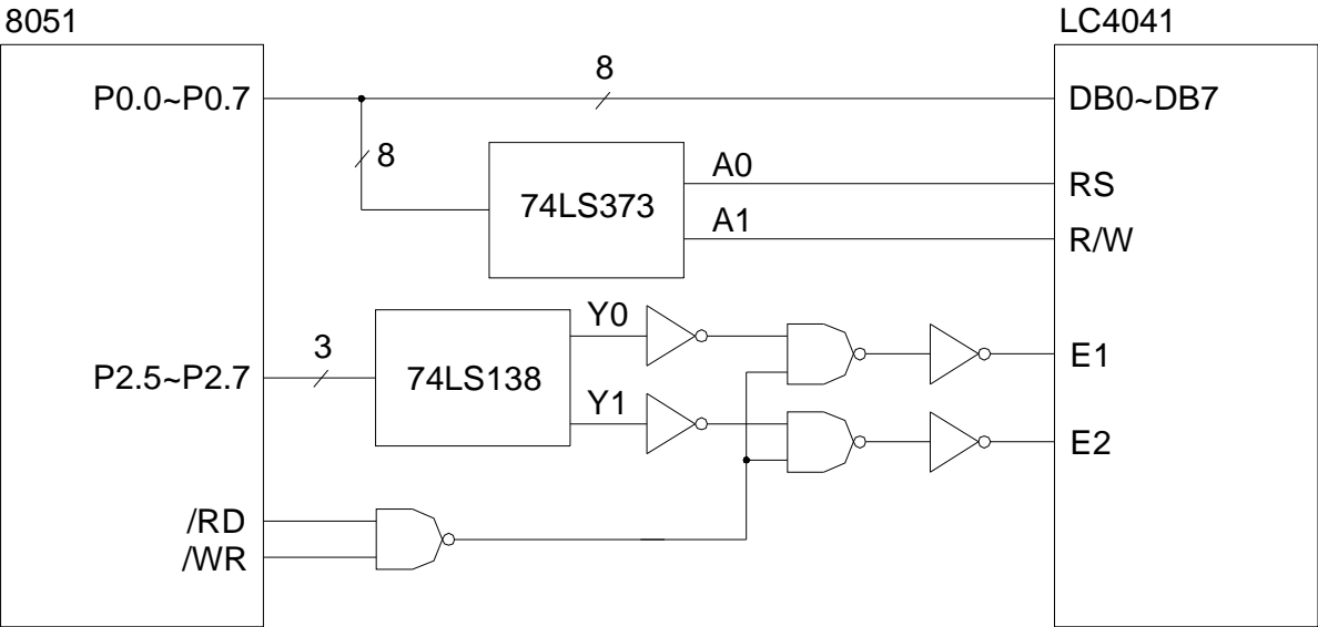
a. Application Circuit 1
