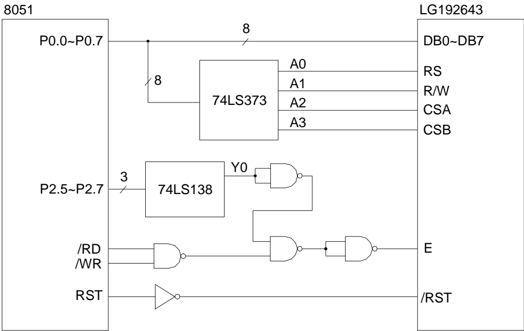
a. Application Circuit 1
